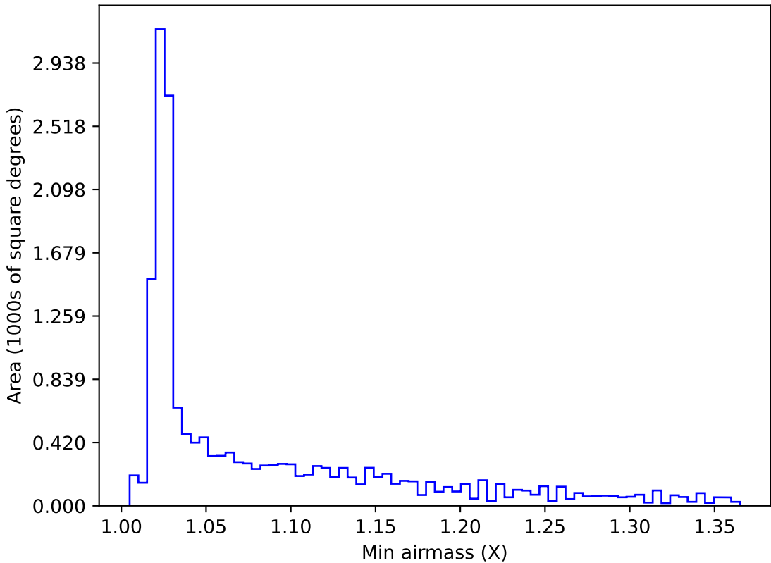
too_elab_r32_d3_ugrizy_v3.4_10yrs WFD all bands: Min airmass
