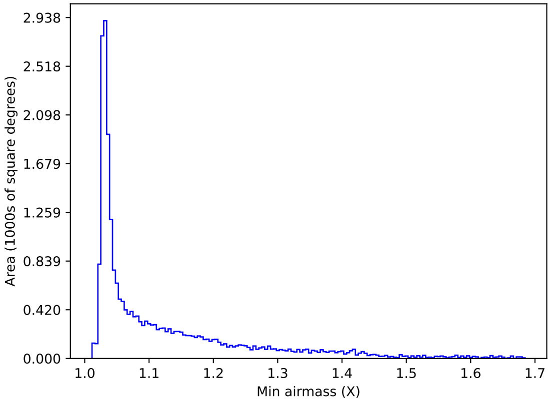
too_elab_r32_d3_ugrizy_v3.4_10yrs All sky y band: Min airmass
