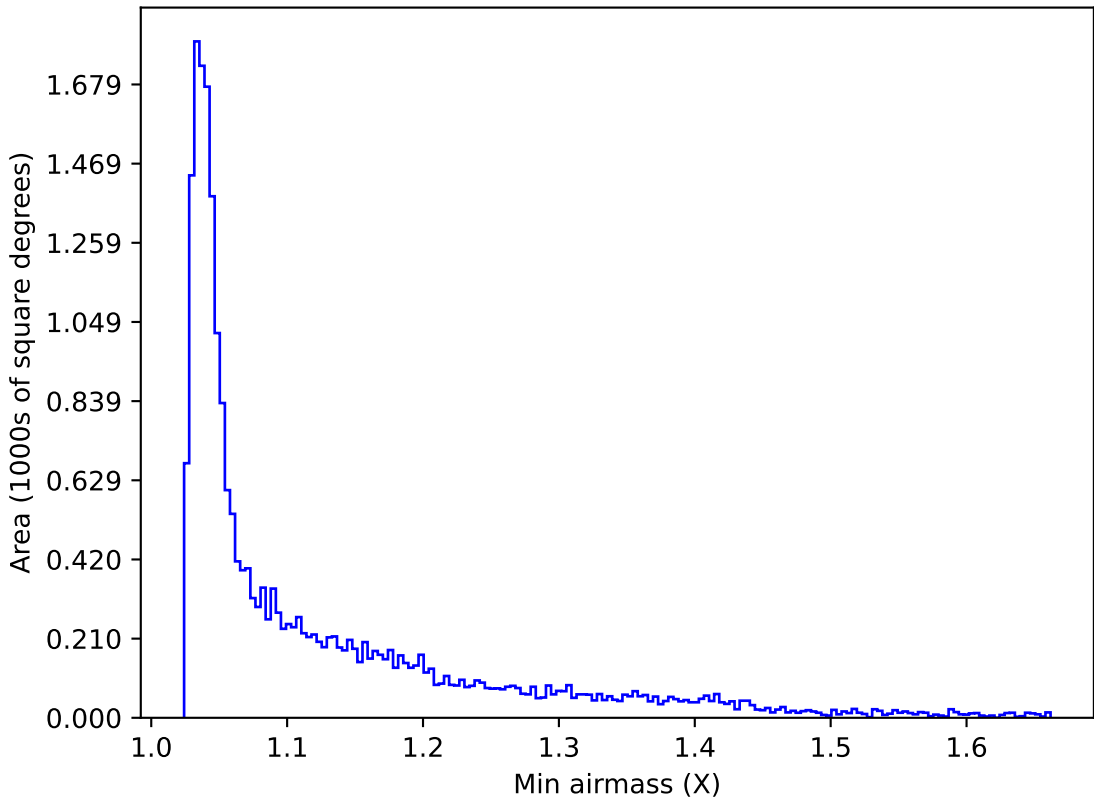
too_elab_r32_d3_ugrizy_v3.4_10yrs All sky u band: Min airmass
