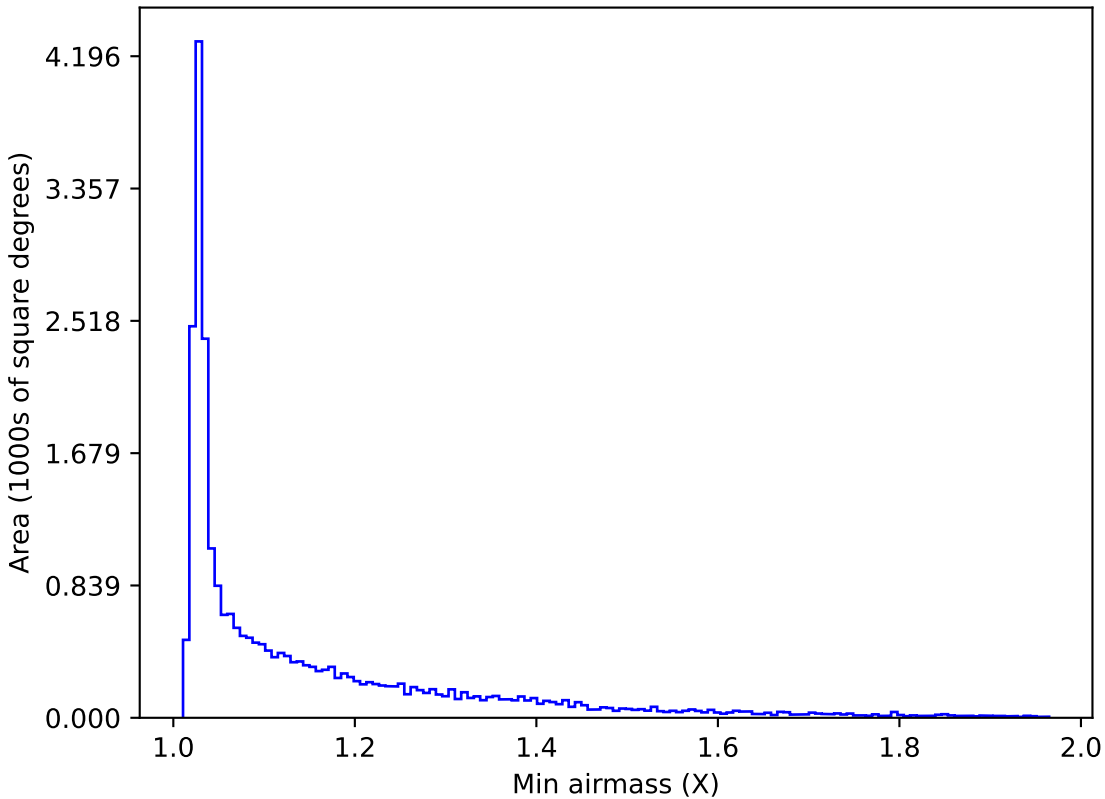
too_elab_r32_d3_ugrizy_v3.4_10yrs All sky r band: Min airmass
