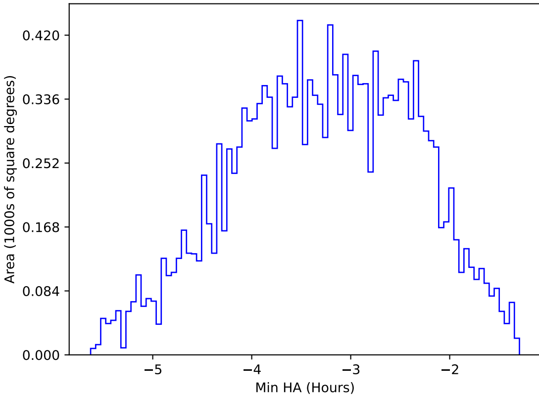
too_elab_r32_d3_ugrizy_v3.4_10yrs WFD u band: Min HA
