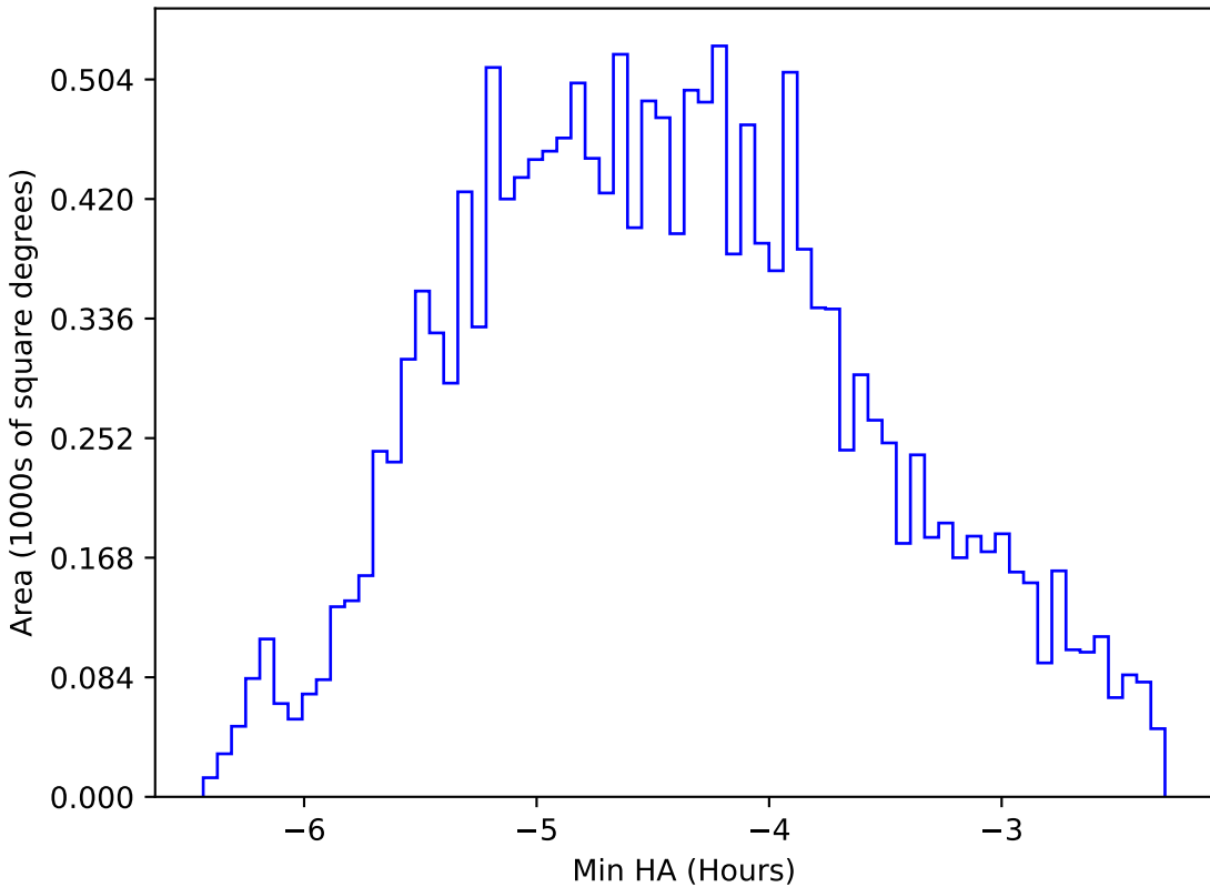
too_elab_r32_d3_ugrizy_v3.4_10yrs WFD r band: Min HA
