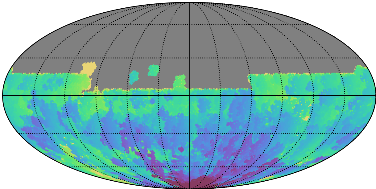
too_elab_r32_d3_ugrizy_v3.4_10yrs All sky u band: Min HA
