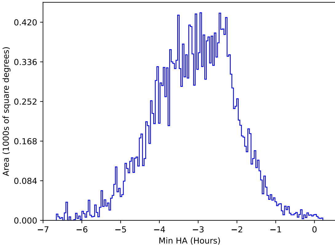
too_elab_r32_d3_uigrizy_v3.4_10yrs All sky u band: Min HA
