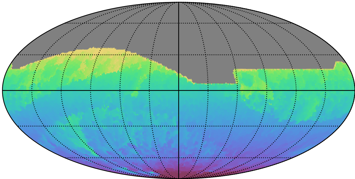
too_elab_r32_d3_ugrizy_v3.4_10yrs All sky all bands: Min HA
