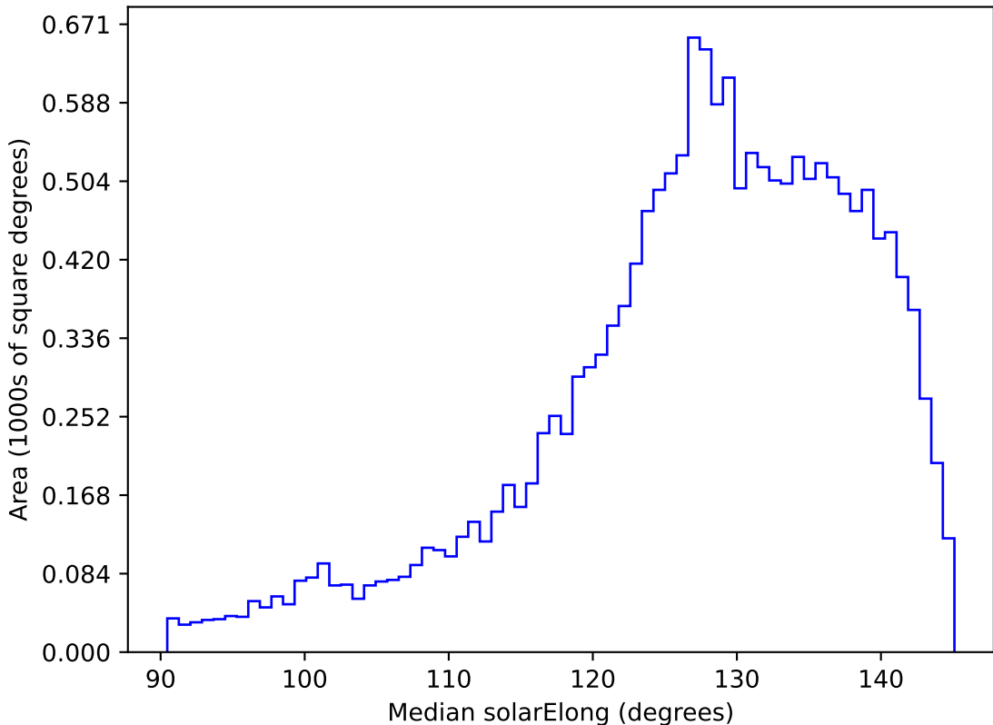
too_elab_r32_d3_ugrizy_v3.4_10yrs WFD z band: Median solarElong
