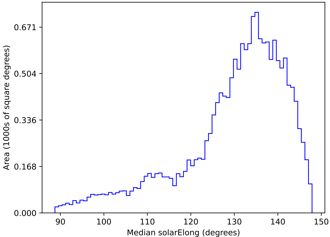
too_elab_r32_d3_ugrizy_v3.4_10yrs WFD y band: Median solarElong
