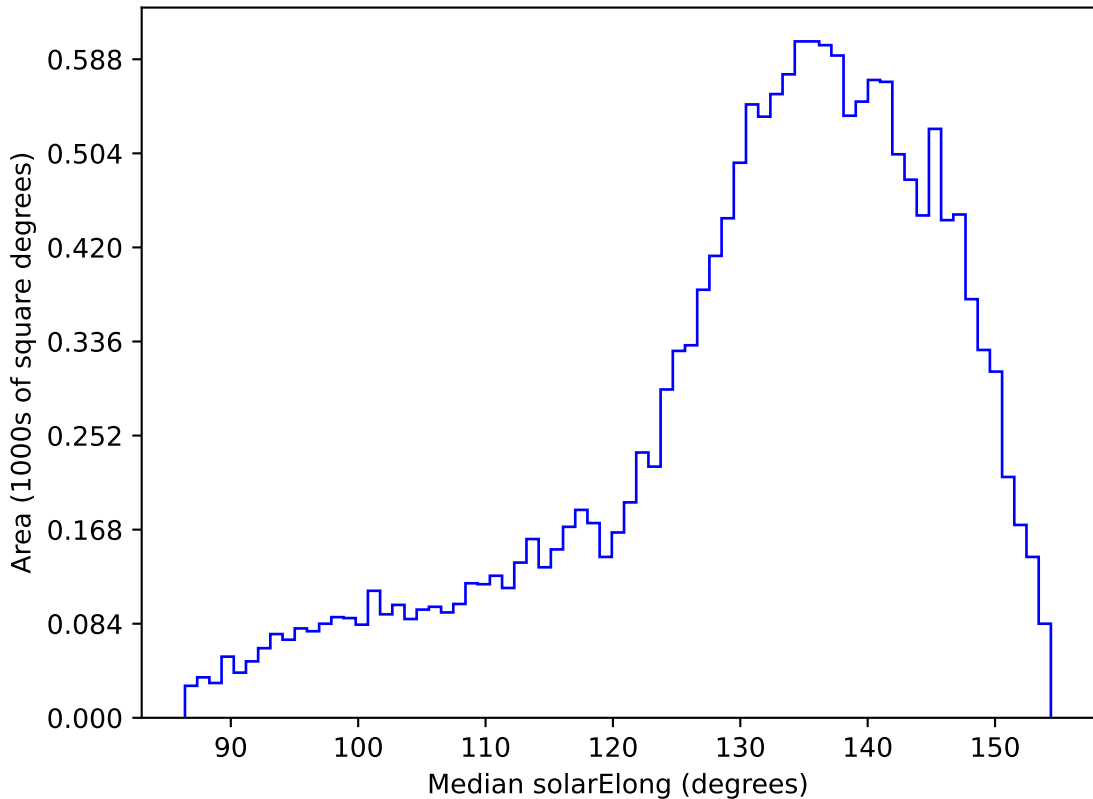
too_elab_r32_d3_ugrizy_v3.4_10yrs WFD u band: Median solarElong
