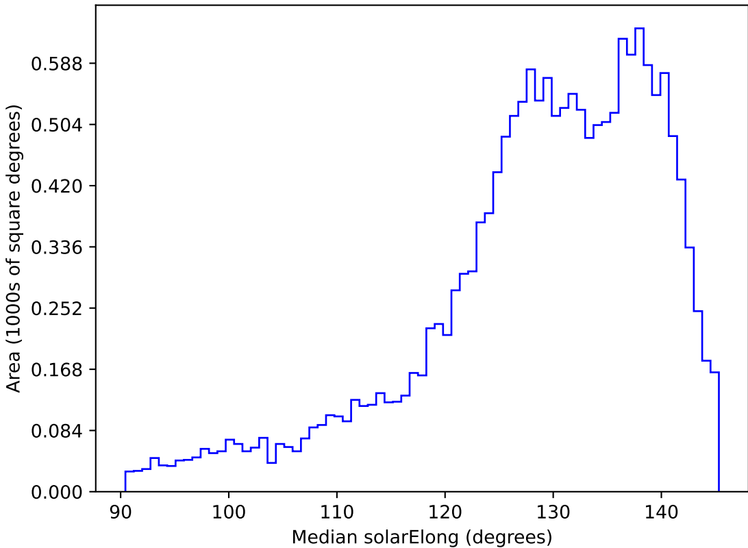
too_elab_r32_d3_ugrizy_v3.4_10yrs WFD i band: Median solarElong
