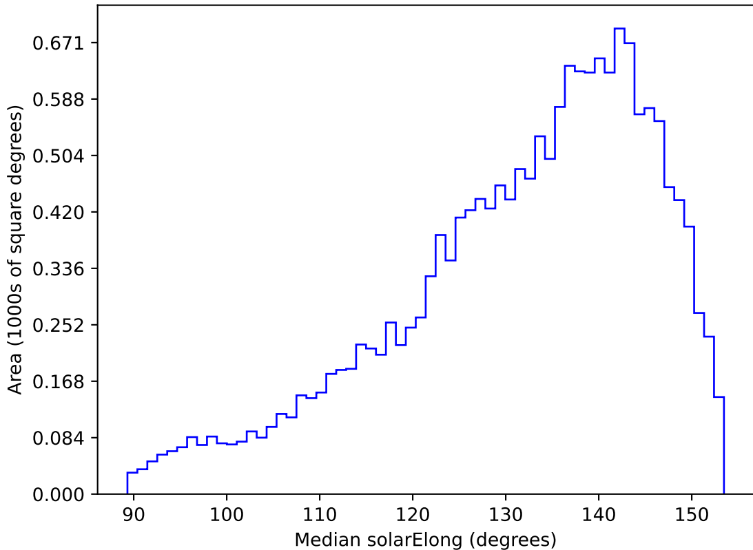
too_elab_r32_d3_ugrizy_v3.4_10yrs WFD g band: Median solarElong
