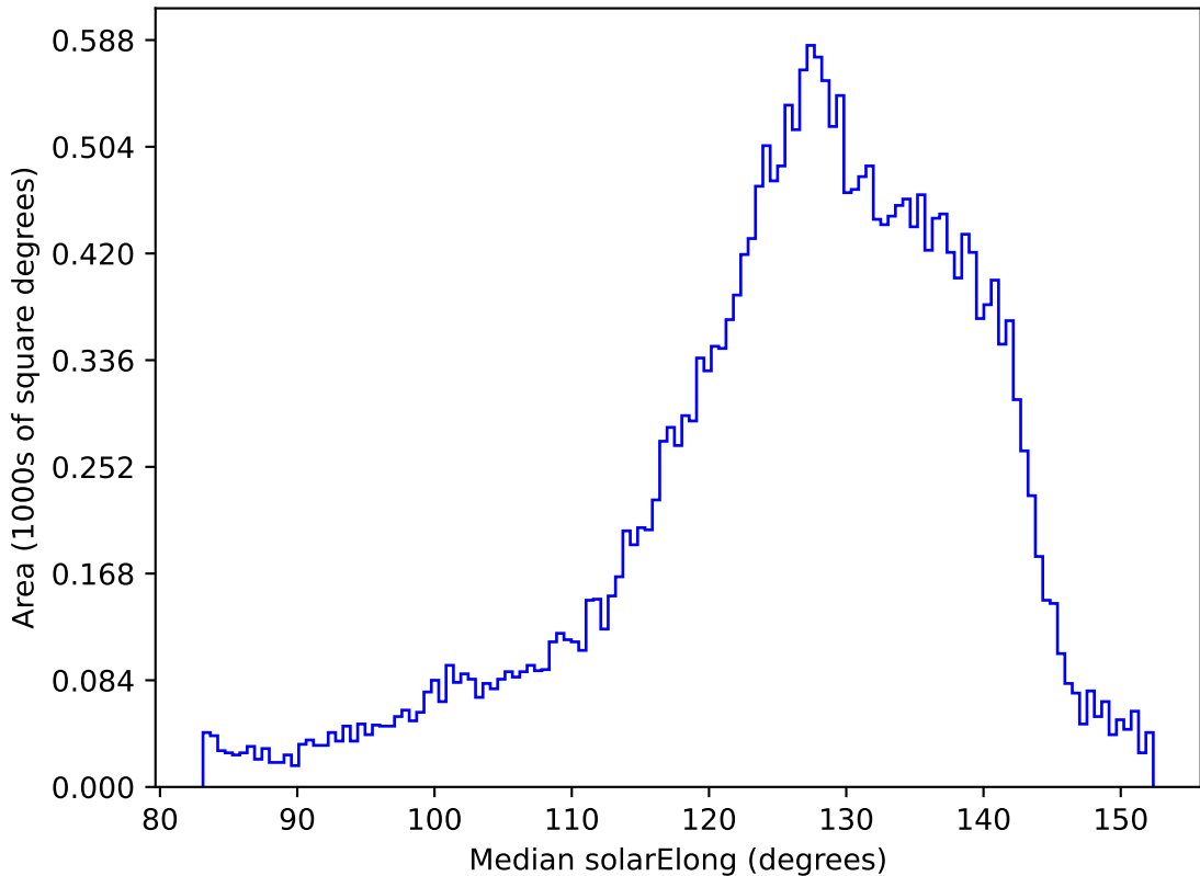
too_elab_r32_d3_ugrizy_v3.4_10yrs All sky z band: Median solarElong
