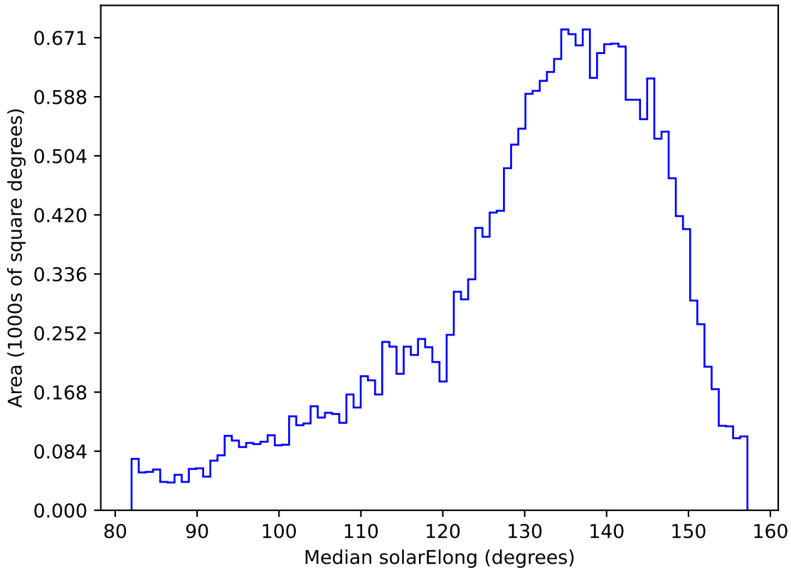
too_elab_r32_d3_ugrizy_v3.4_10yrs All sky u band: Median solarElong
