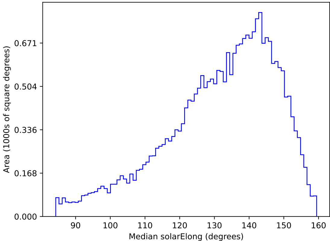
too_elab_r32_d3_ugrizy_v3.4_10yrs All sky g band: Median solarElong
