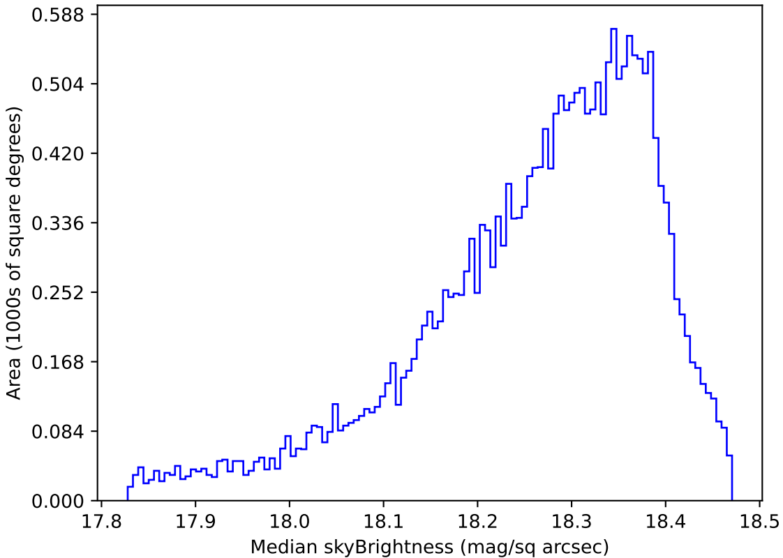
too_elab_r32_d3_ugrizy_v3.4_10yrs Yr 1 y band: Median skyBrightness
