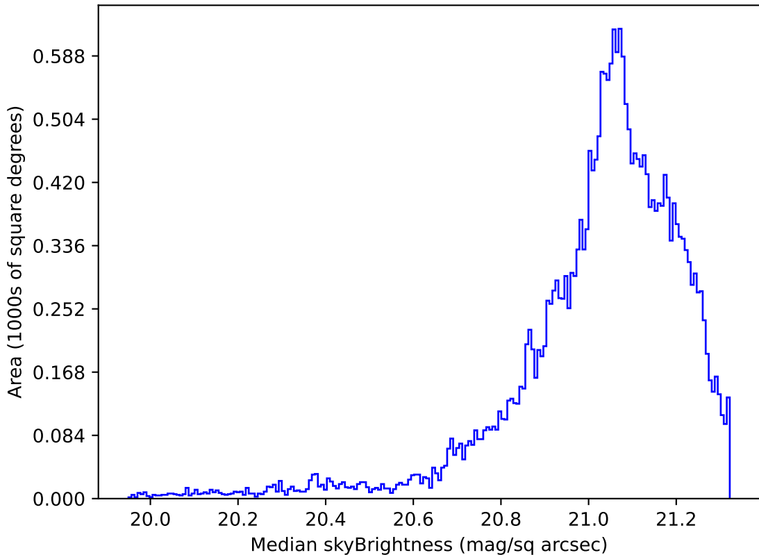
too_elab_r32_d3_ugrizy_v3.4_10yrs Yr 1 r band: Median skyBrightness
