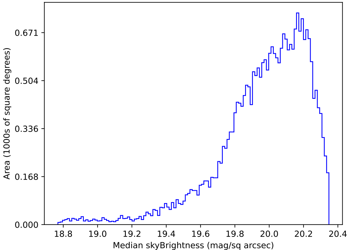
too_elab_r32_d3_ugrizy_v3.4_10yrs Yr 1 i band: Median skyBrightness
