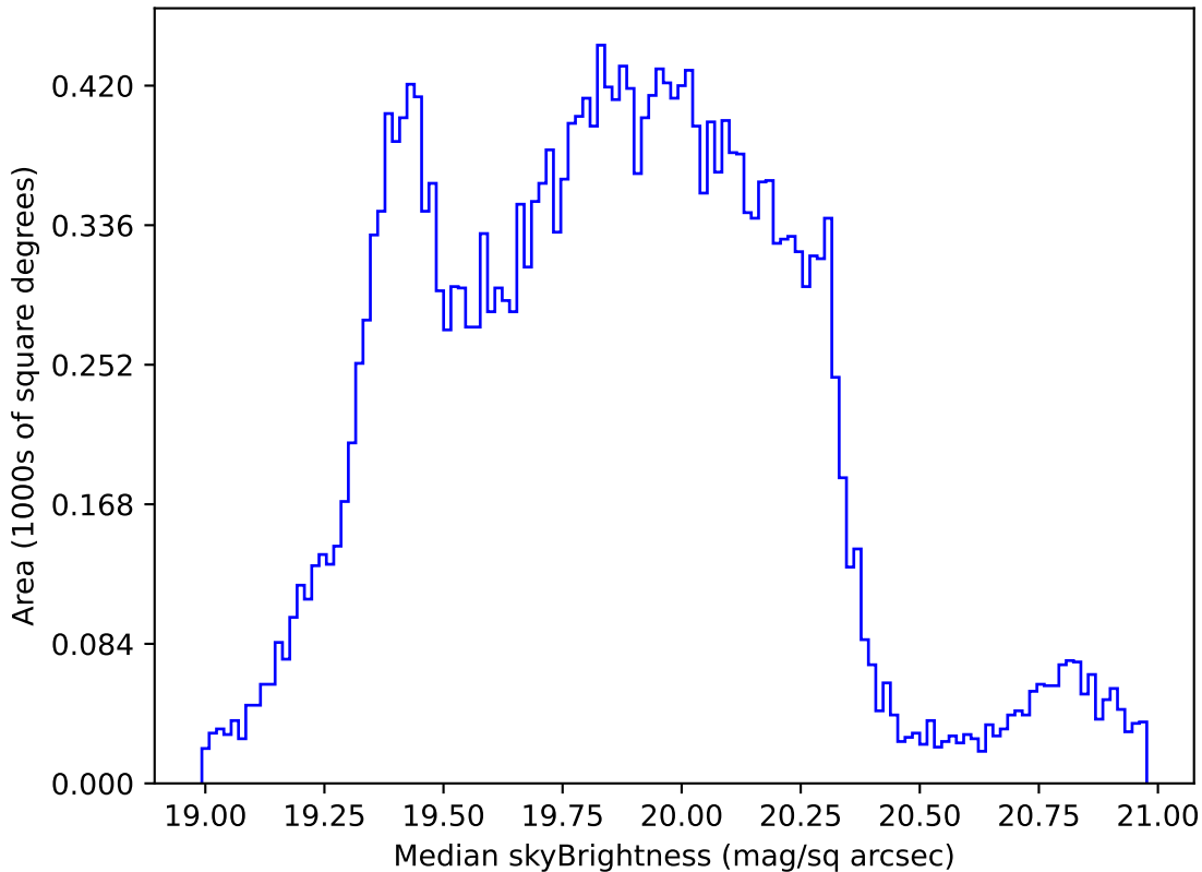
too_elab_r32_d3_ugrizy_v3.4_10yrs Yr 1 all bands: Median skyBrightness
