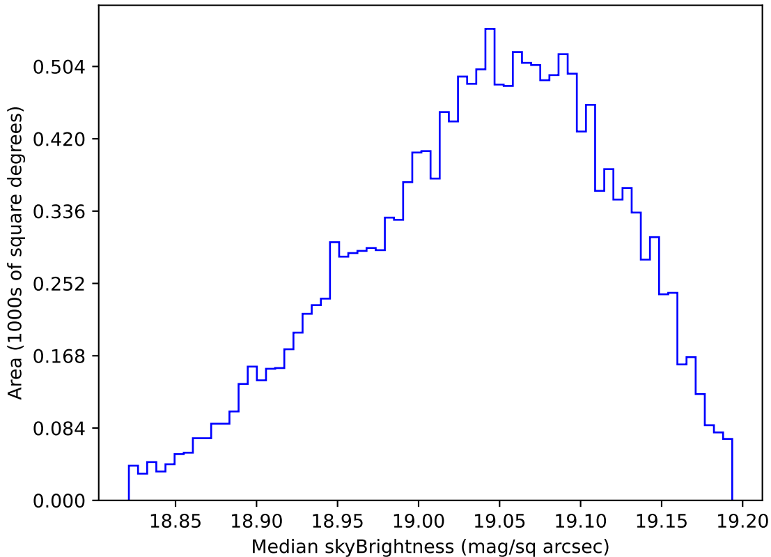
too_elab_r32_d3_ugrizy_v3.4_10yrs WFD z band: Median skyBrightness
