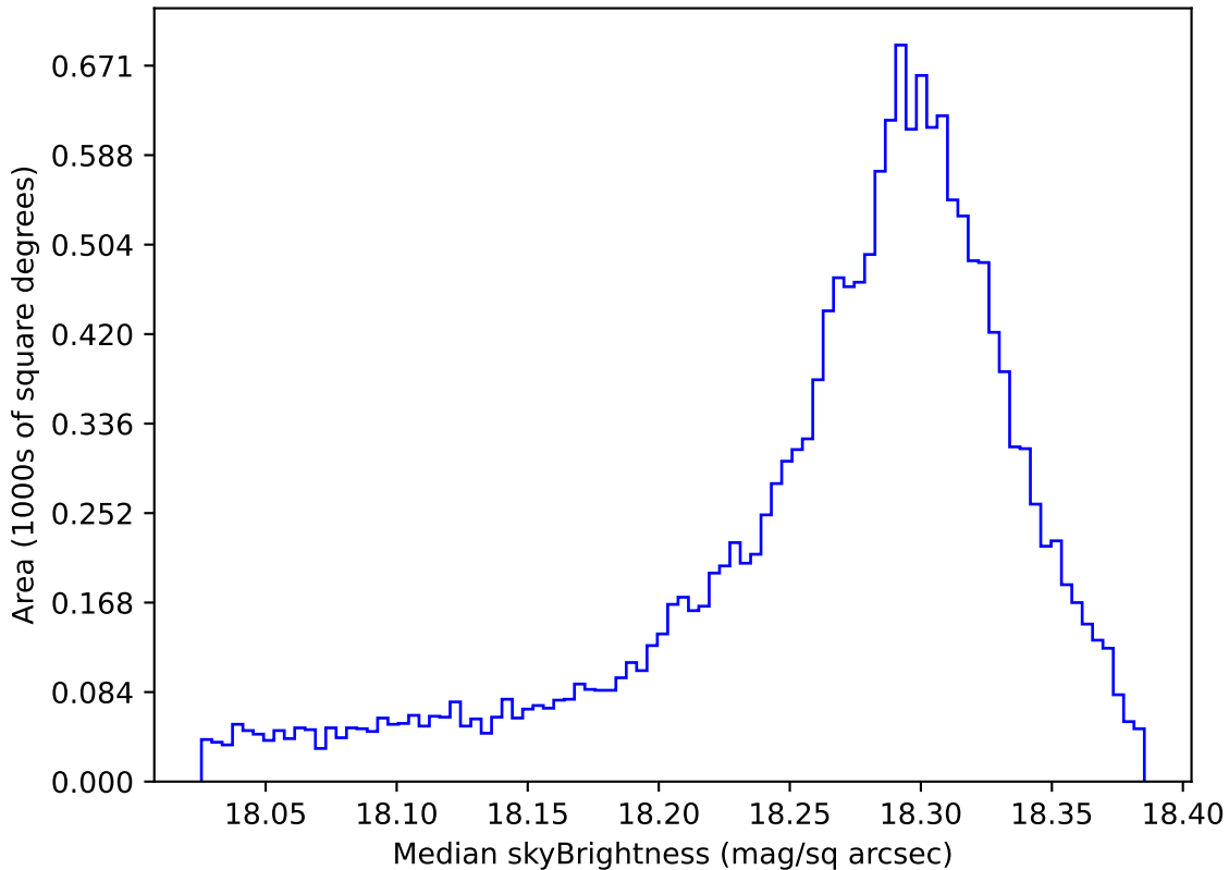
too_elab_r32_d3_ugrizy_v3.4_10yrs WFD y band: Median skyBrightness
