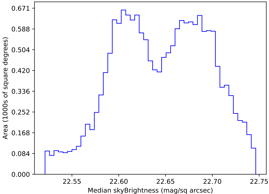
too_elab_r32_d3_ugrizy_v3.4_10yrs WFD u band: Median skyBrightness
