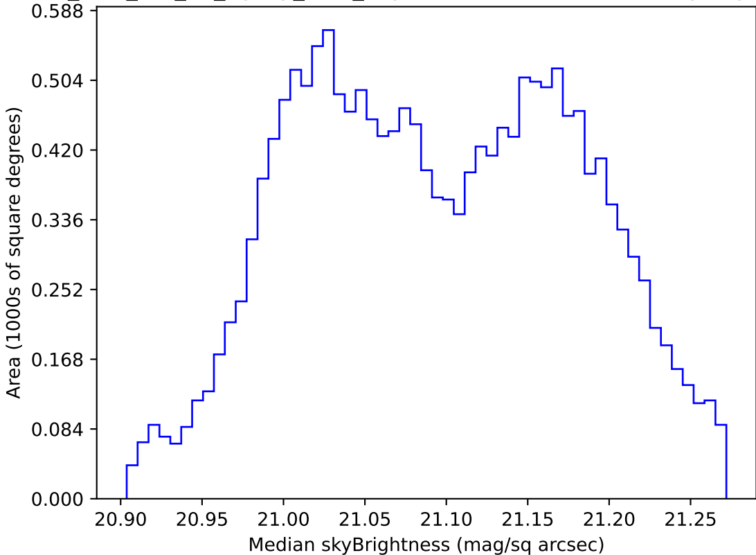
too_elab_r32_d3_ugrizy_v3.4_10yrs WFD r band: Median skyBrightness
