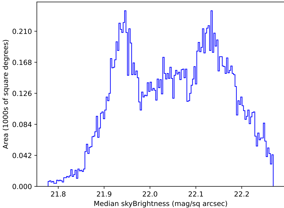
too_elab_r32_d3_ugrizy_v3.4_10yrs WFD g band: Median skyBrightness
