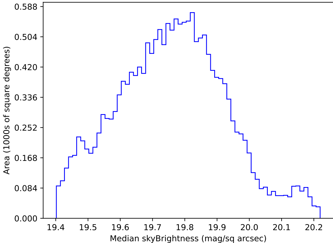
too_elab_r32_d3_ugrizy_v3.4_10yrs WFD all bands: Median skyBrightness
