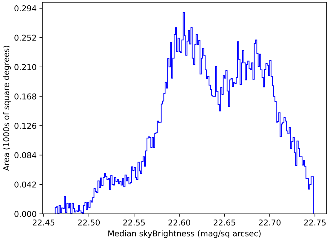
too_elab_r32_d3_ugrizy_v3.4_10yrs All sky u band: Median skyBrightness
