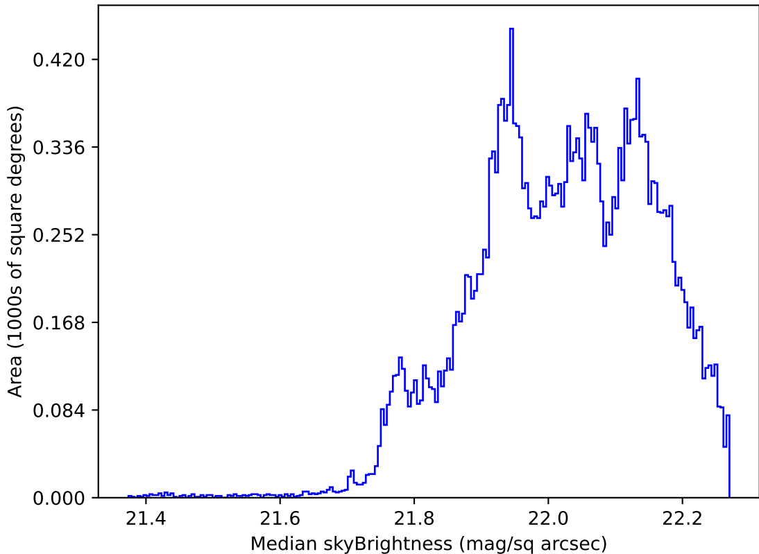
too_elab_r32_d3_ugrizy_v3.4_10yrs All sky g band: Median skyBrightness
