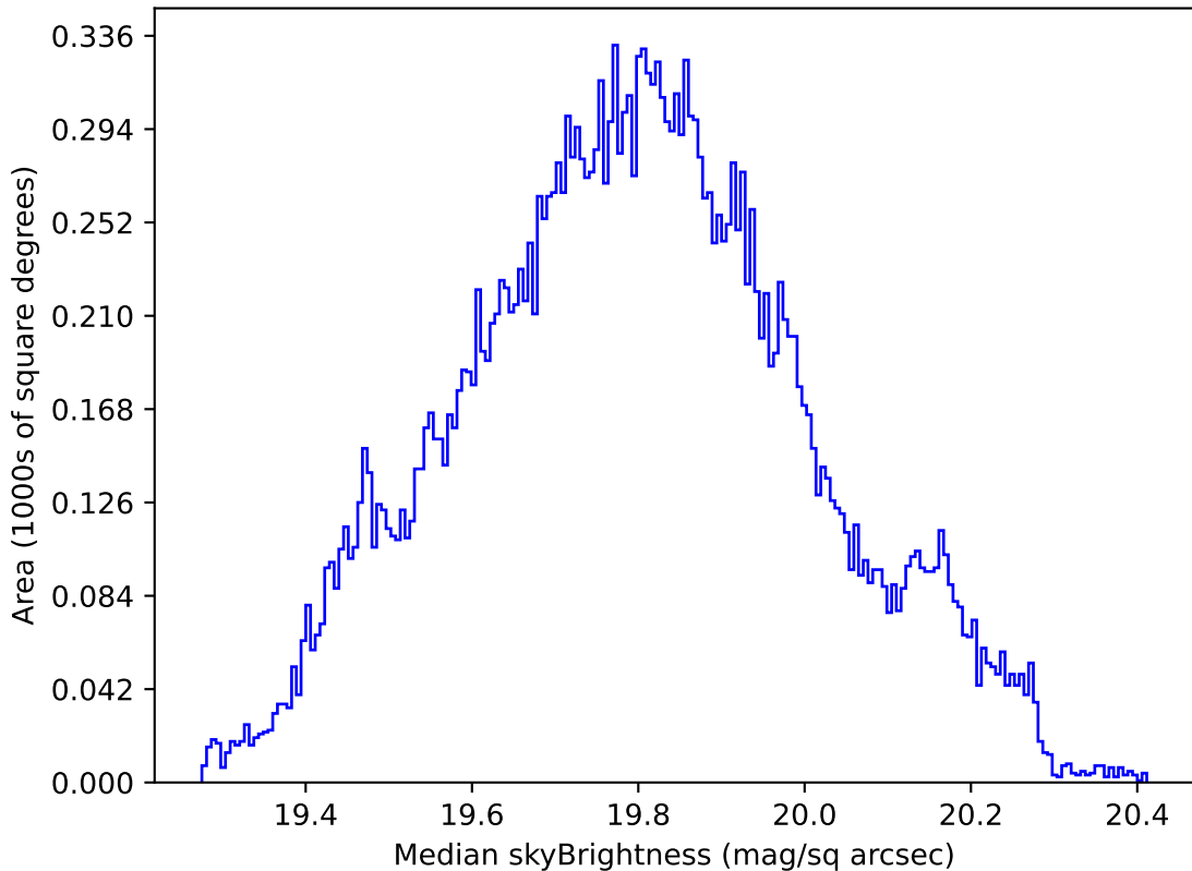
too_elab_r32_d3_ugrizy_v3.4_10yrs All sky all bands: Median skyBrightness
