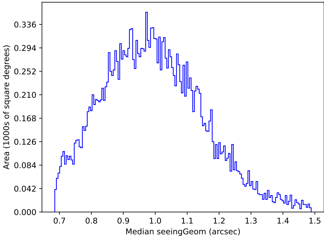
too_elab_r32_d3_ugrizy_v3.4_10yrs Yr 1 u band: Median seeingGeom
