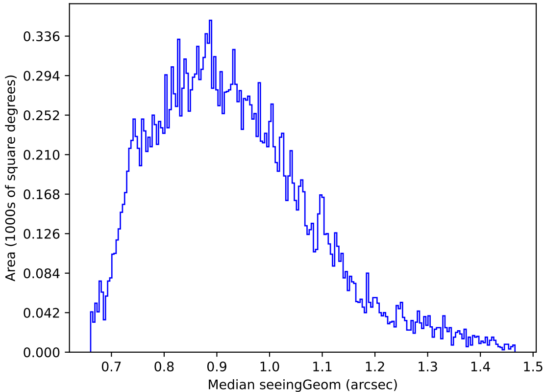
too_elab_r32_d3_ugrizy_v3.4_10yrs Yr 1 g band: Median seeingGeom
