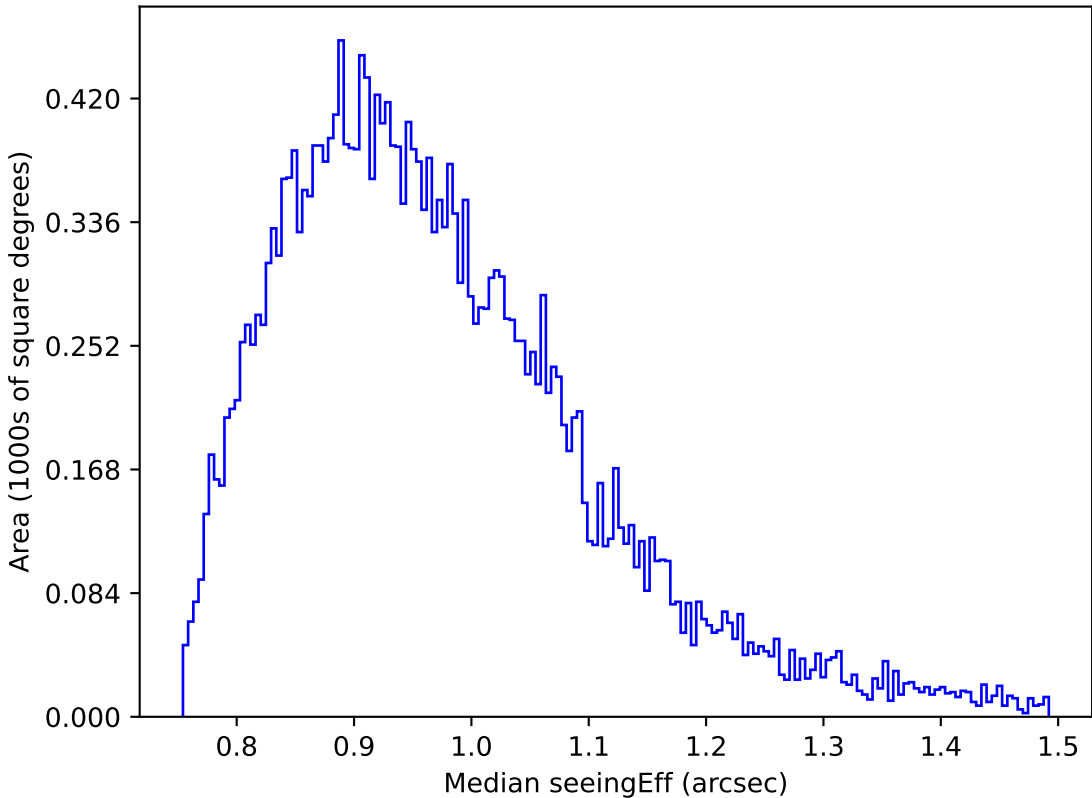
too_elab_r32_d3_ugrizy_v3.4_10yrs Yr 1 z band: Median seeingEff
