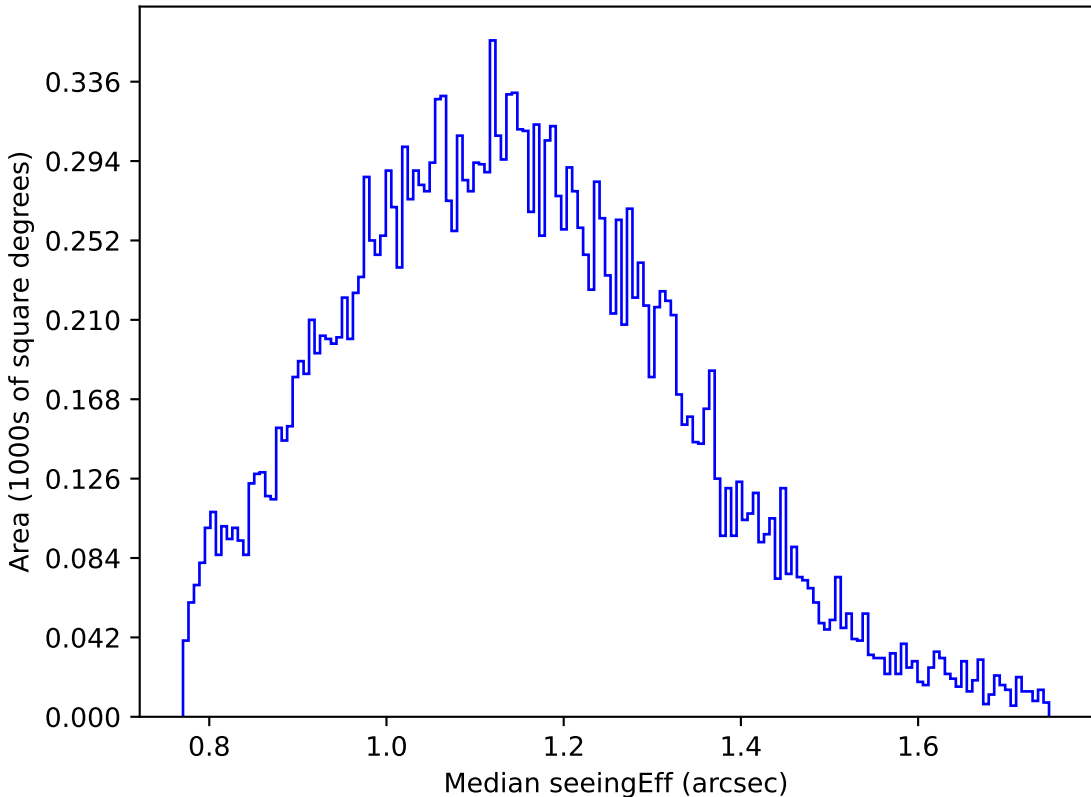
too_elab_r32_d3_ugrizy_v3.4_10yrs Yr 1 u band: Median seeingEff
