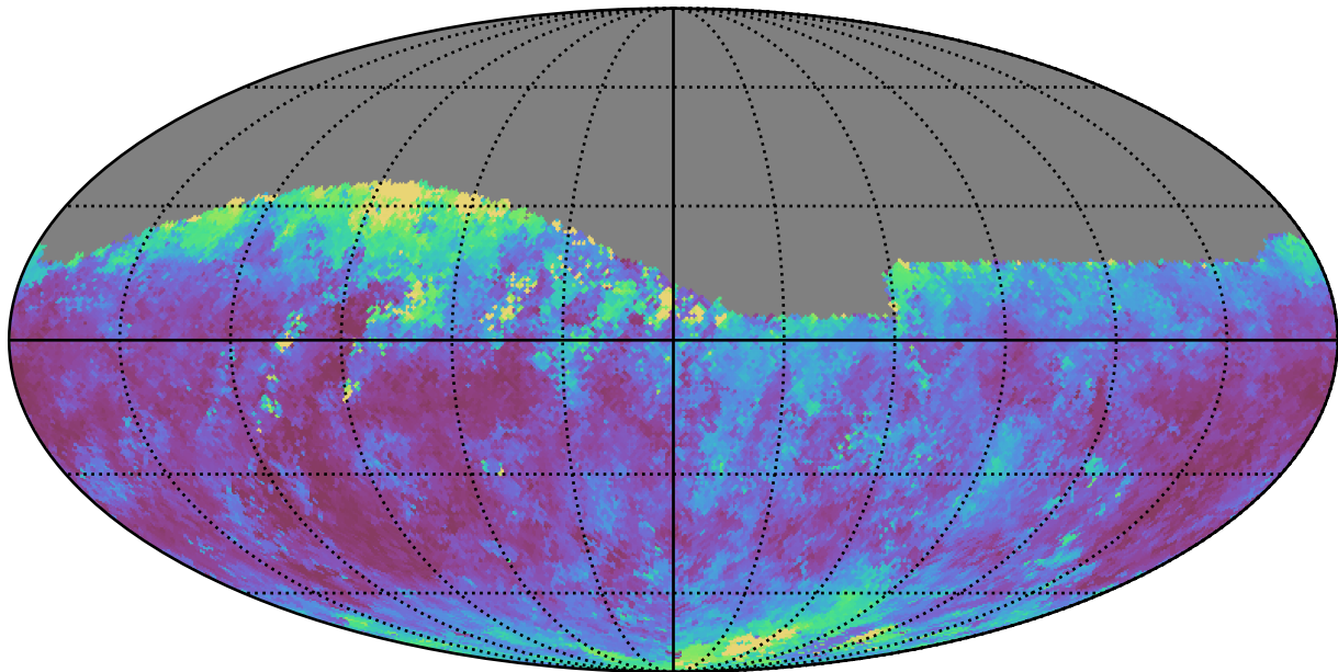
too_elab_r32_d3_ugrizy_v3.4_10yrs Yr 1 r band: Median seeingEff
