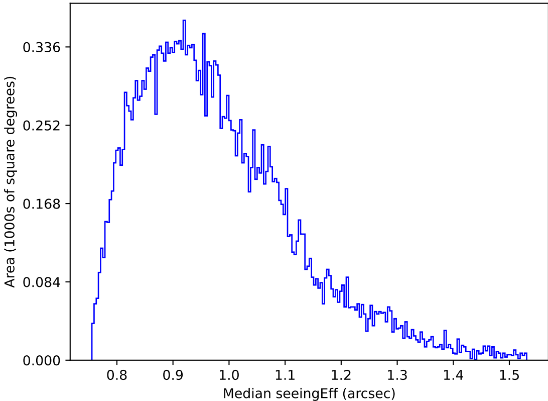
too_elab_r32_d3_ugrizy_v3.4_10yrs Yr 1 r band: Median seeingEff
