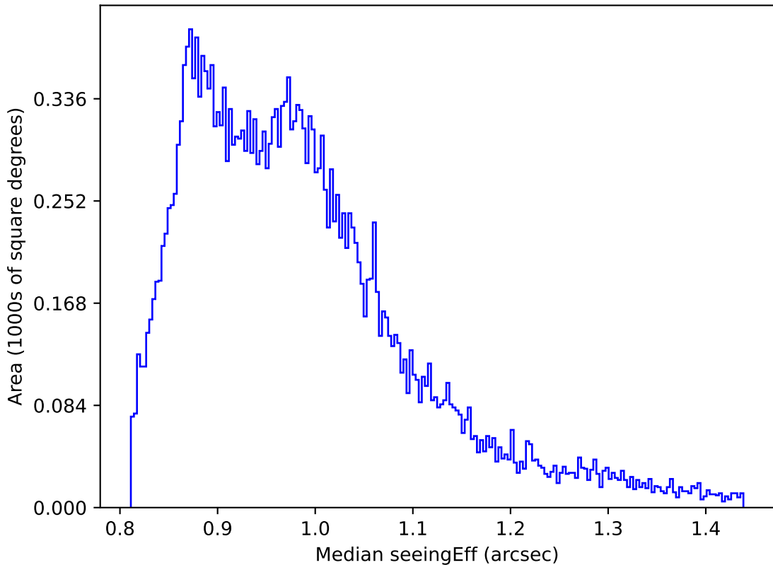
too_elab_r32_d3_ugrizy_v3.4_10yrs Yr 1 all bands: Median seeingEff
