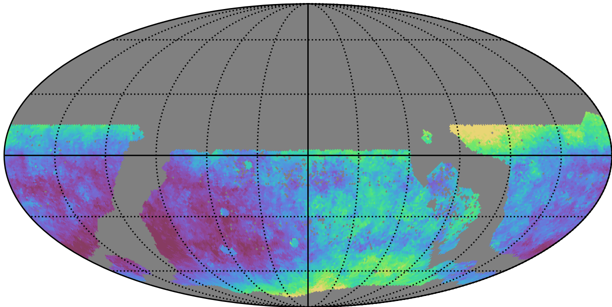
too_elab_r32_d3_ugrizy_v3.4_10yrs WFD z band: Median seeingEff
