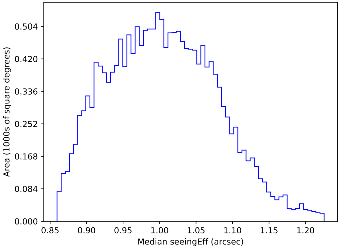
too_elab_r32_d3_ugrizy_v3.4_10yrs WFD z band: Median seeingEff
