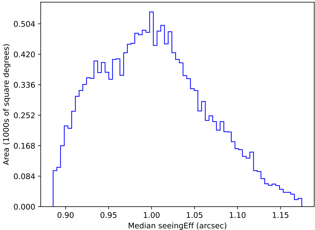
too_elab_r32_d3_ugrizy_v3.4_10yrs WFD y band: Median seeingEff
