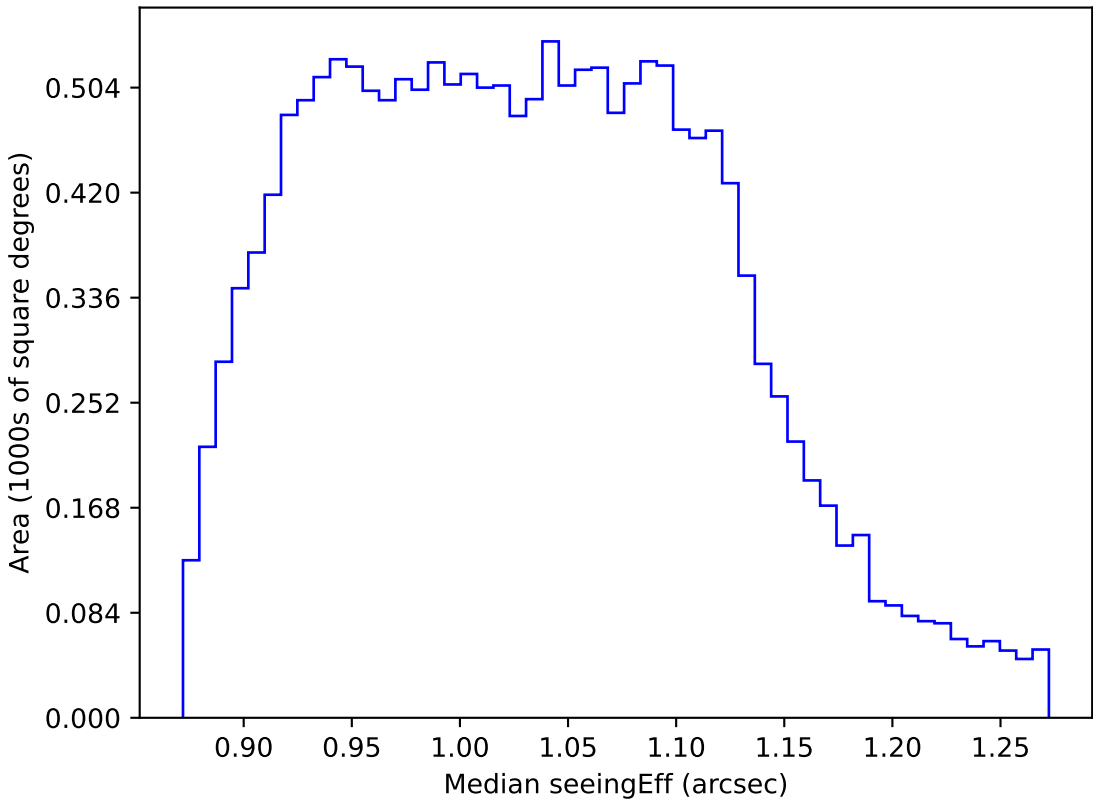
too_elab_r32_d3_ugrizy_v3.4_10yrs WFD r band: Median seeingEff
