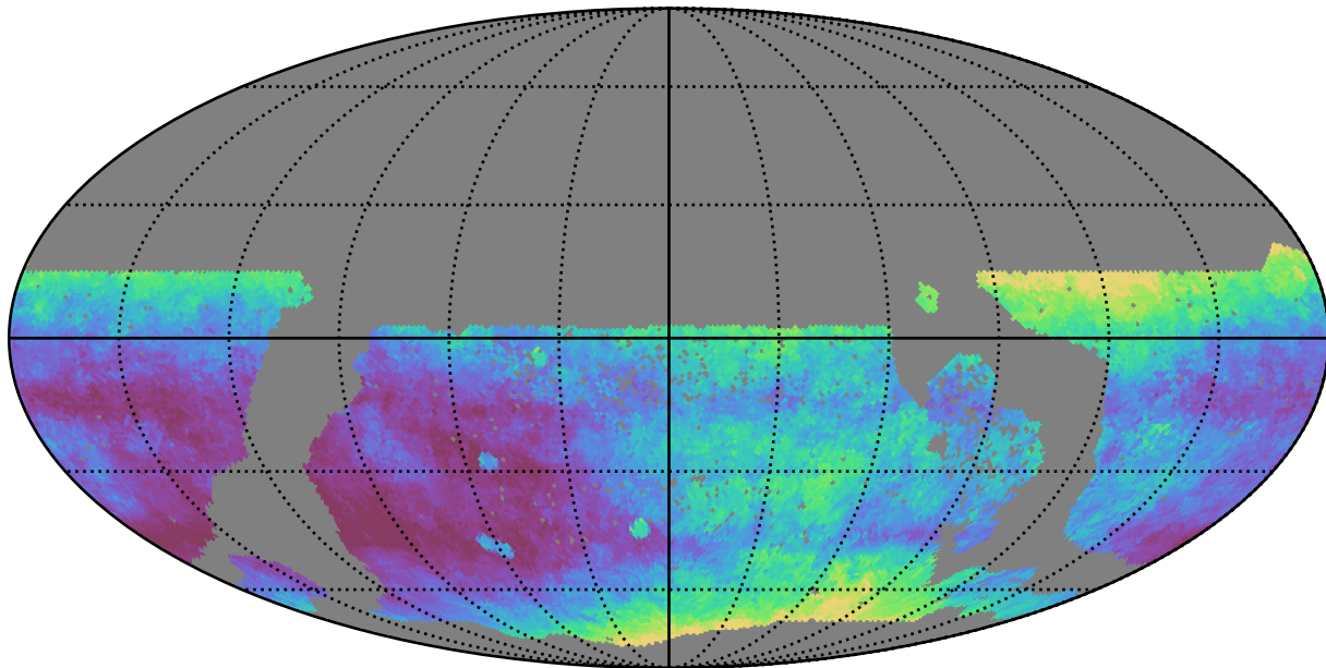
too_elab_r32_d3_ugrizy_v3.4_10yrs WFD i band: Median seeingEff
