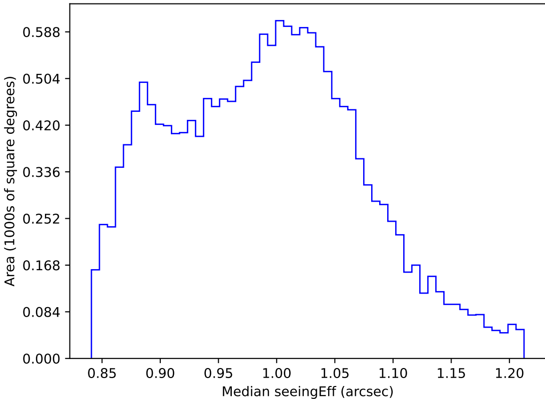
too_elab_r32_d3_ugrizy_v3.4_10yrs WFD i band: Median seeingEff
