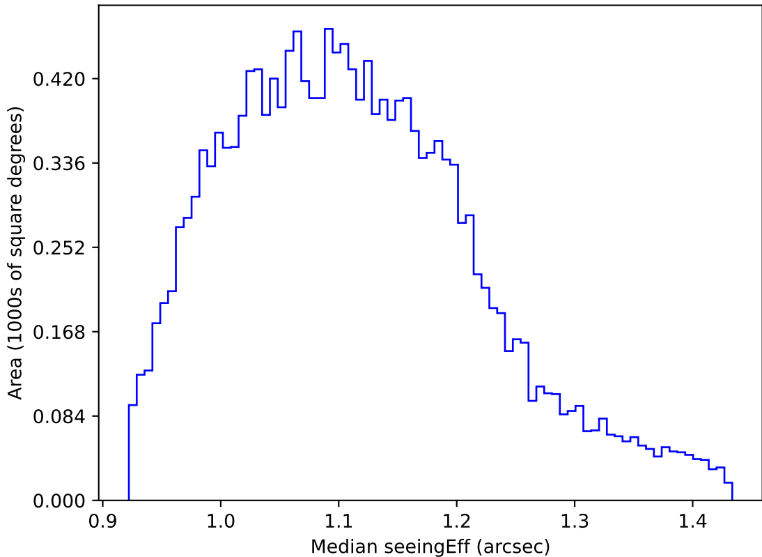
too_elab_r32_d3_ugrizy_v3.4_10yrs WFD g band: Median seeingEff
