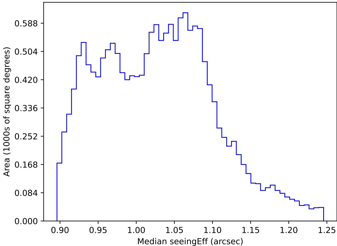
too_elab_r32_d3_ugrizy_v3.4_10yrs WFD all bands: Median seeingEff
