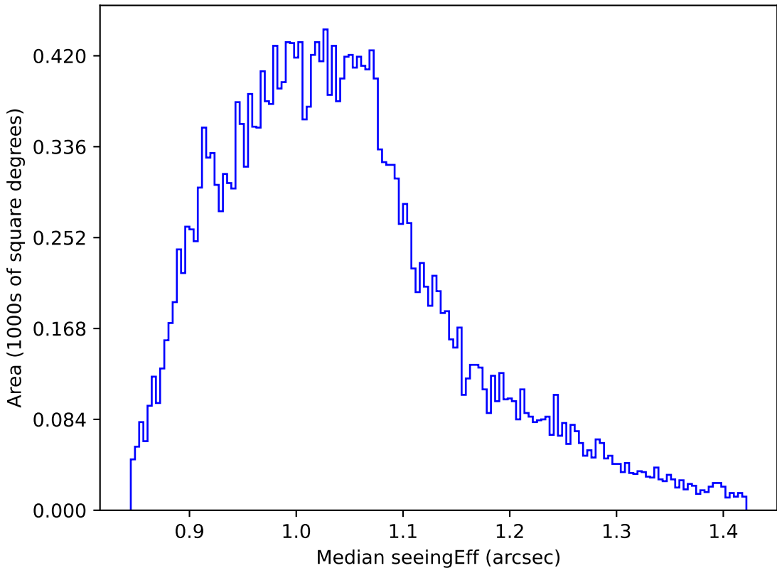
too_elab_r32_d3_ugrizy_v3.4_10yrs All sky z band: Median seeingEff
