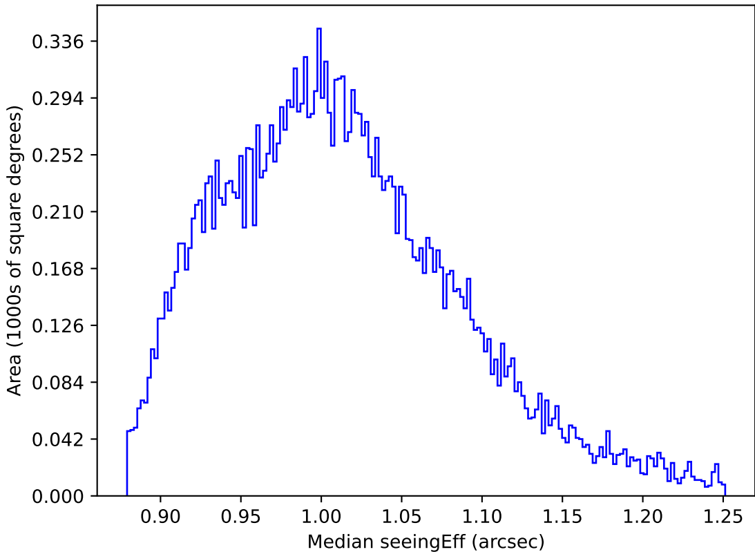
too_elab_r32_d3_ugrizy_v3.4_10yrs All sky y band: Median seeingEff
