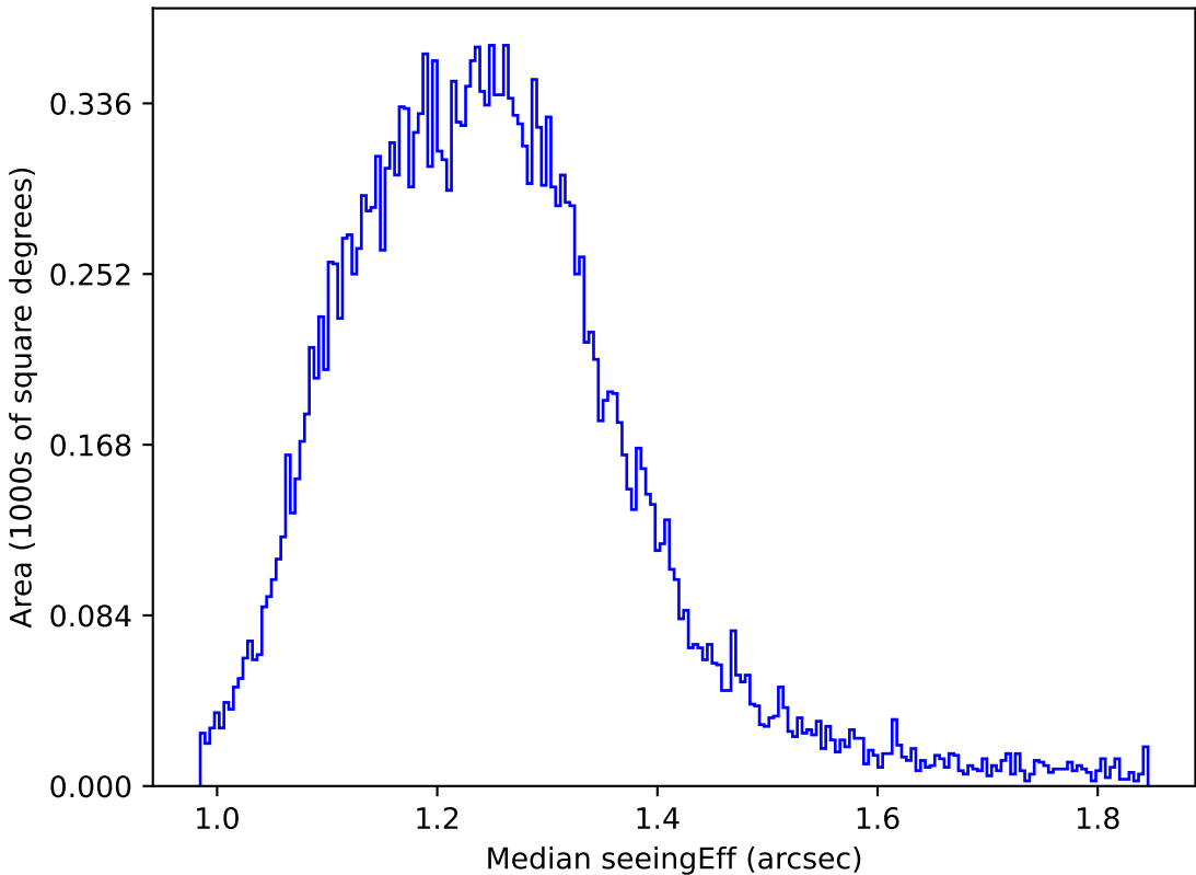
too_elab_r32_d3_ugrizy_v3.4_10yrs All sky u band: Median seeingEff
