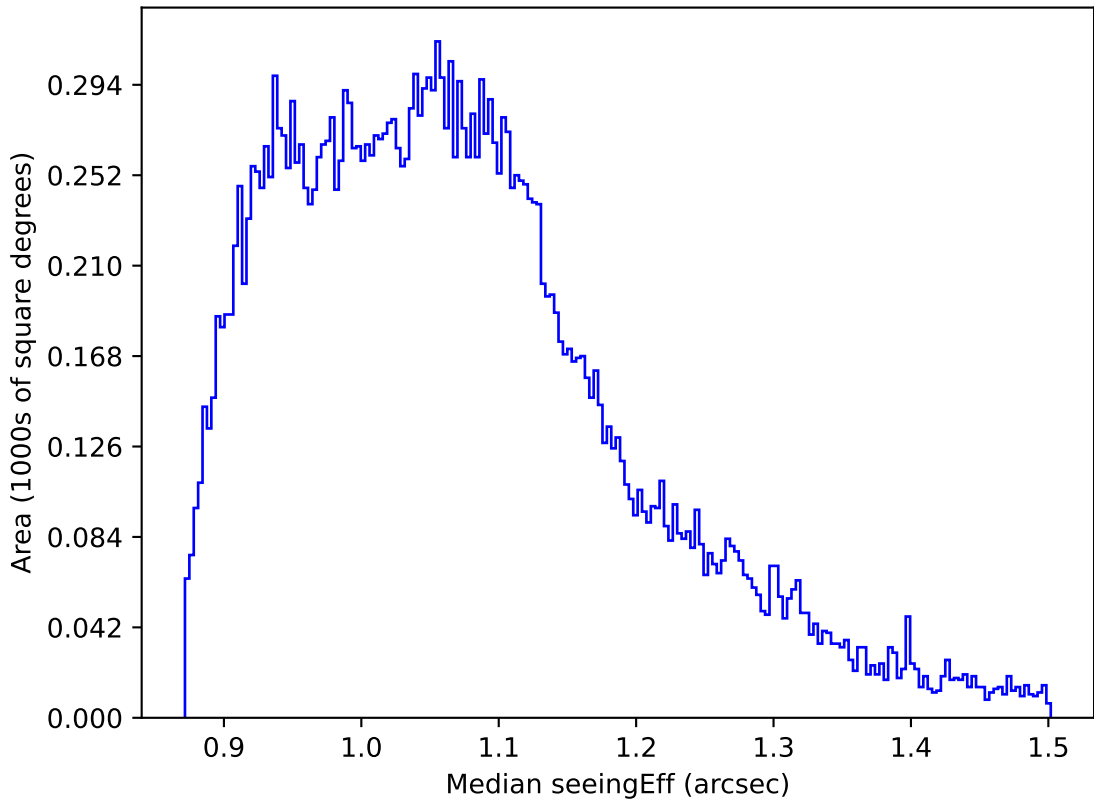
too_elab_r32_d3_ugrizy_v3.4_10yrs All sky r band: Median seeingEff
