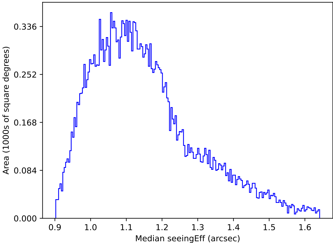
too_elab_r32_d3_ugrizy_v3.4_10yrs All sky g band: Median seeingEff
